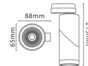
ZR-M3010RA-12W
